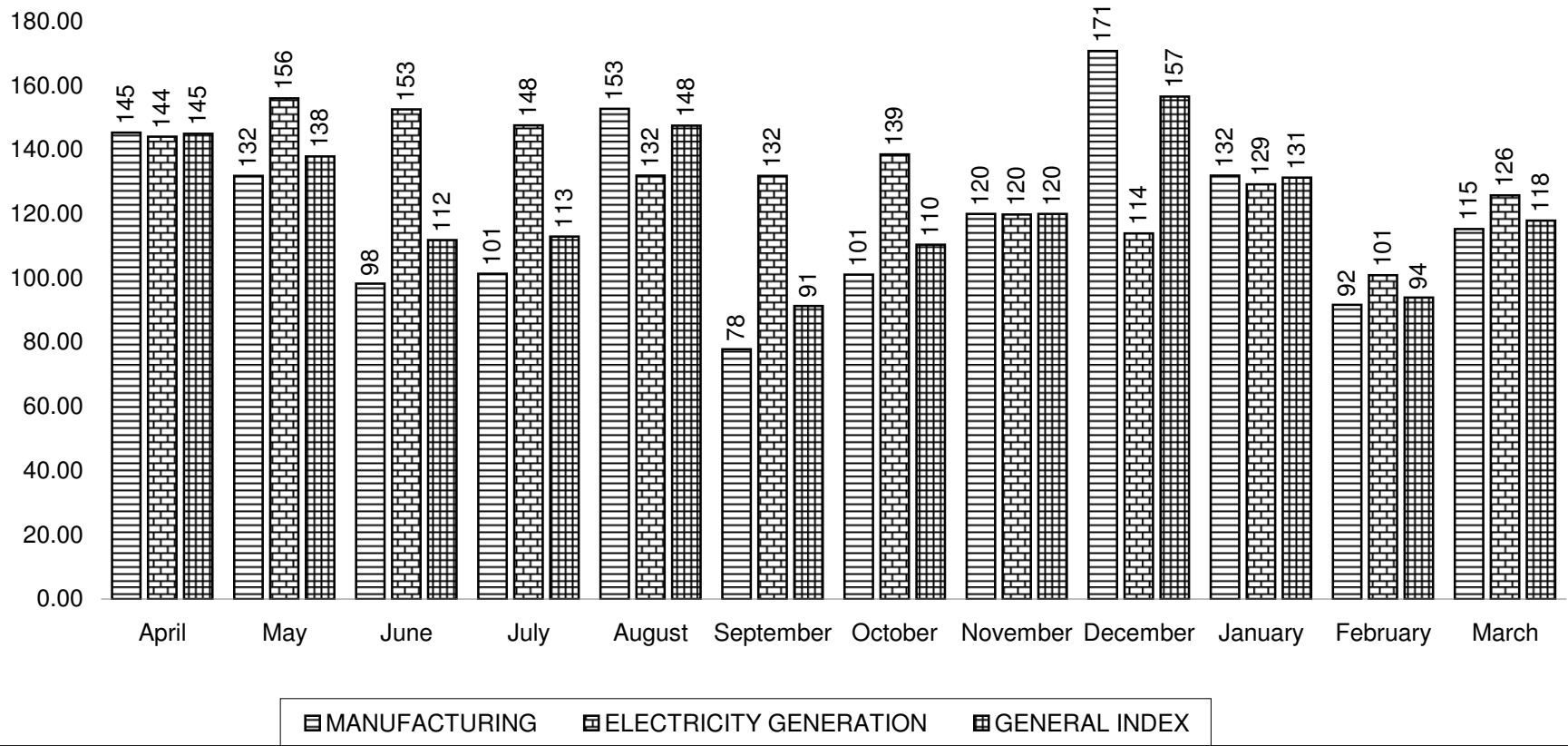
[G-2] INDEX OF INDUSTRIAL PRODUCTION 2009-10 (BASE : 1999-2000)
