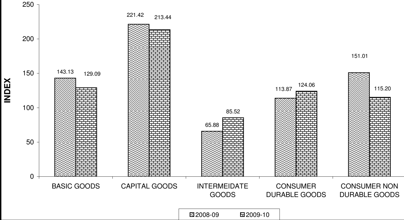
(G-4) GRAPHICAL REPRESENTATION OF IIP AS PER USE BASED CLASSIFICATION
