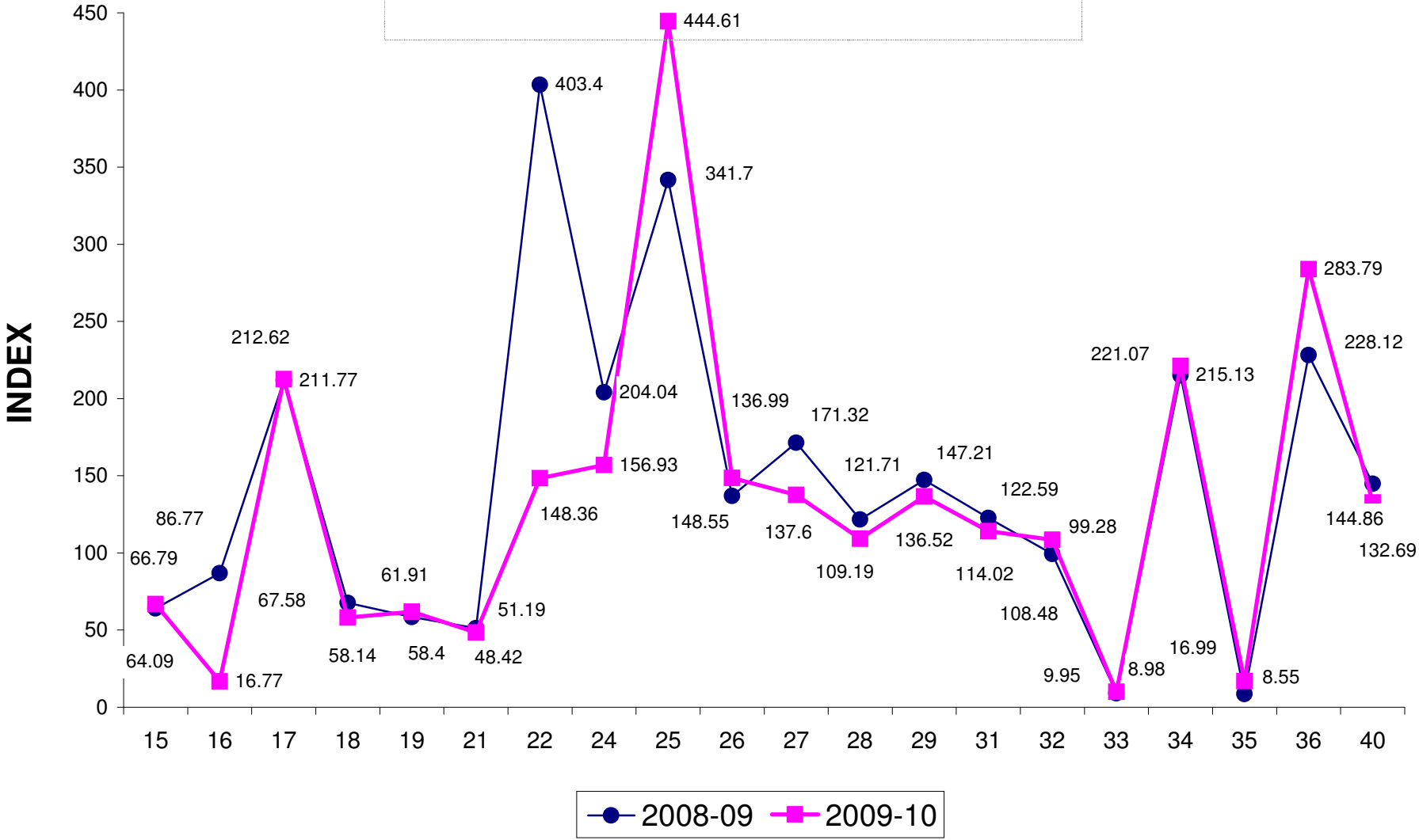
(G-3) INDEX ON INDUSTRIAL PRODUCTION 2008-09 & 2009-10 BASE YEAR: 1999-2000 AT 2 DIGIT LEVEL OF NIC- 1998
